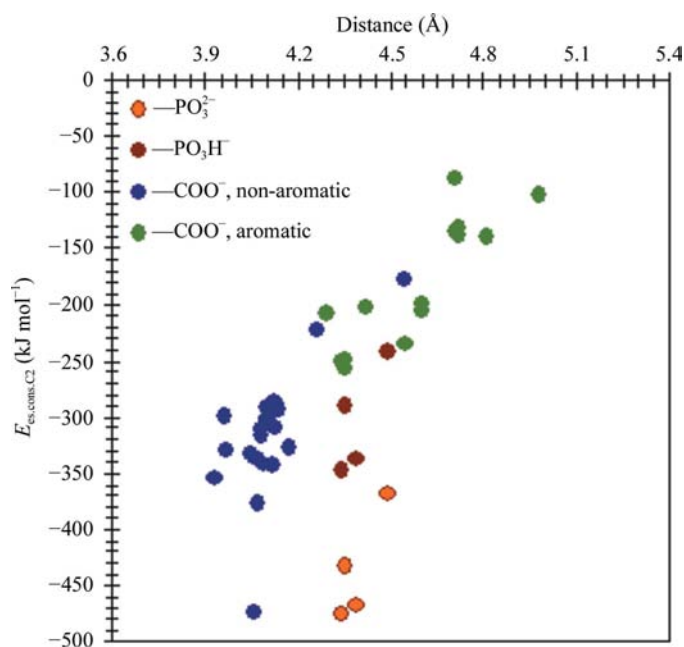
Figure 6 Relation between the electrostatic interaction energy of the C2-group of the inhibitor with the conserved residues of neuraminidase, E_{es,cons,C2} , and the distance between the C2-group of inhibitor and the central Arg371 in the arginine pocket. Distances shown are between the carboxylic C atom or P atom of the C2-group and the CZ C atom of Arg371.
